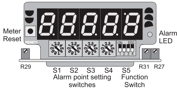
FIG. 1 8901S FRONT VIEW (COVER REMOVED)
